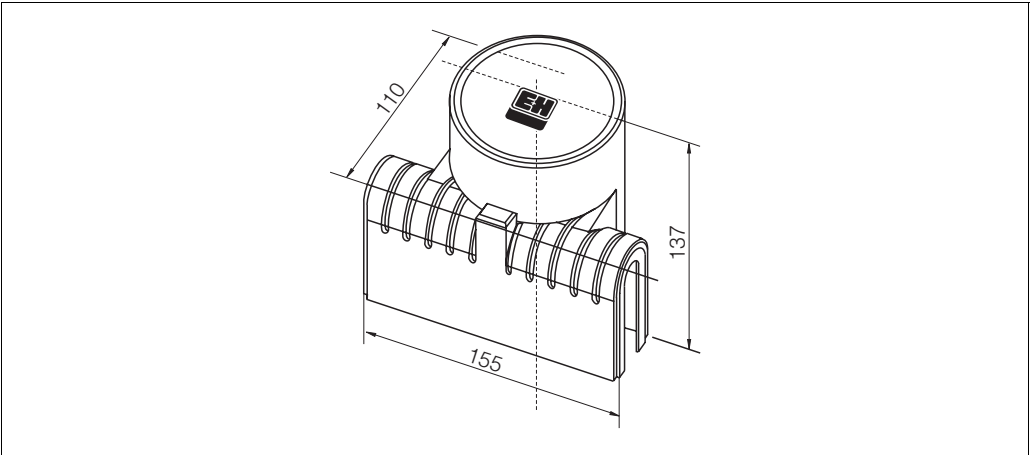
Protection cover
