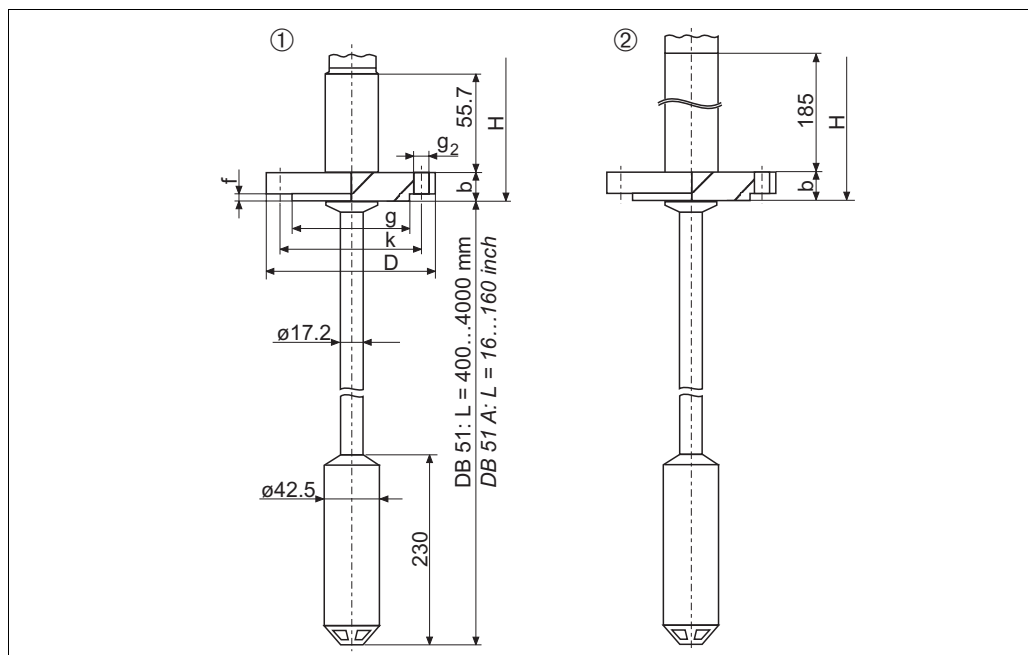
DB51(A), rod version with flange
