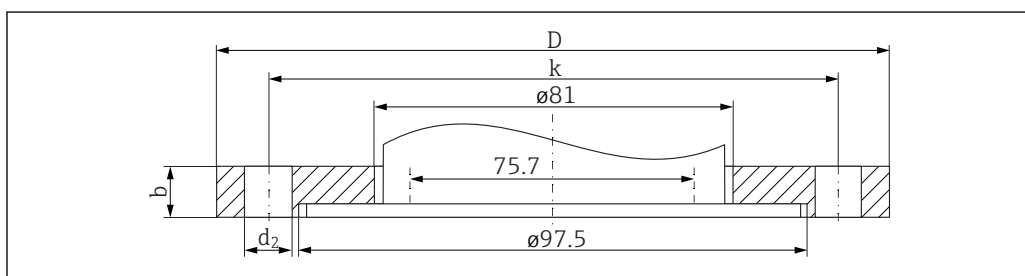
16 Dimensions of FAU80 slip-on flange without adapter flange
