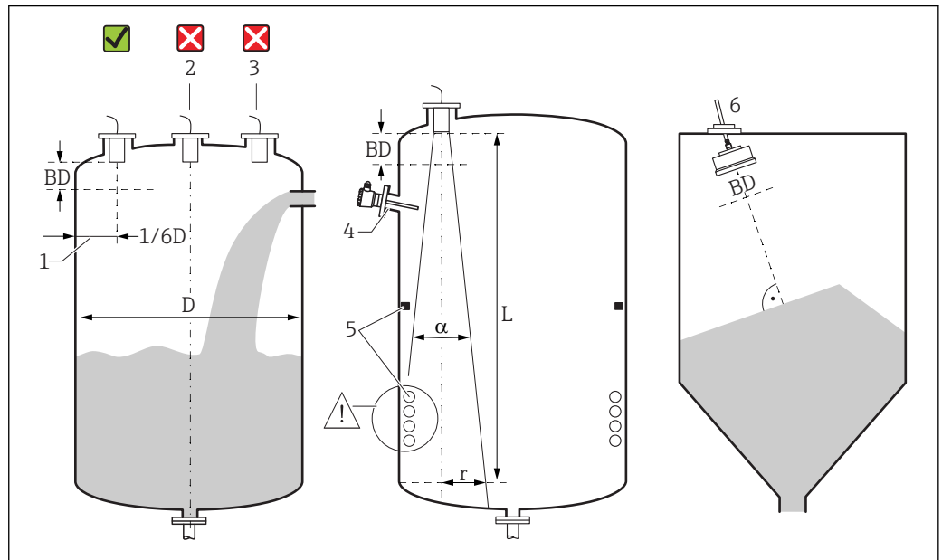
8 Installation conditions for level measurement
