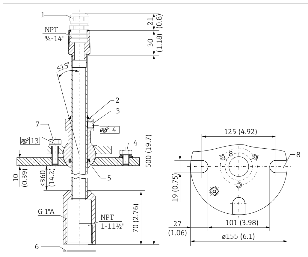
40 FAU40 alignment unit. Unit of measurement mm (in)
