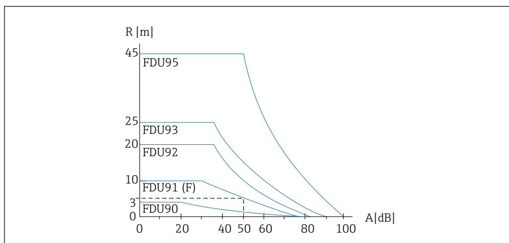
4 Range chart for ultrasonic sensors
