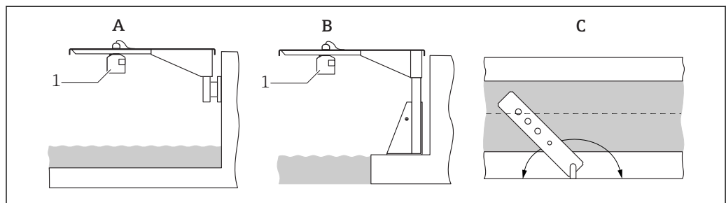
12 Installation with cantilever arm over open channels or flumes
