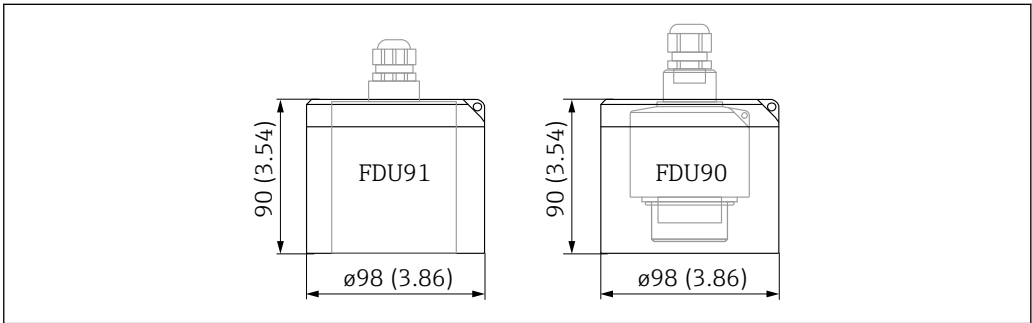
32 Weather protection cover for FDU90/FDU91. Unit of measurement mm (in)
