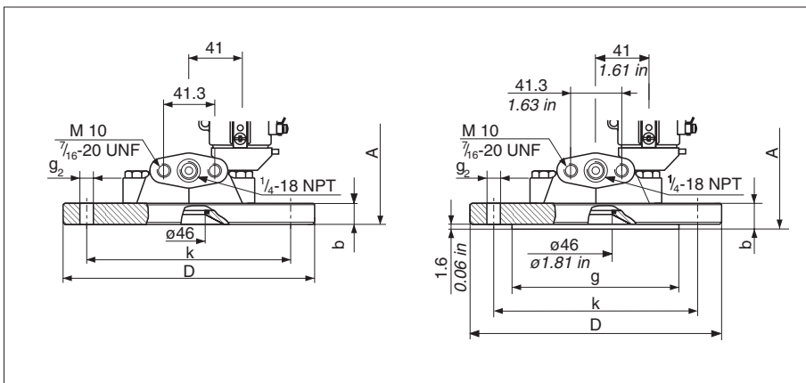
EN flange, connection dimensions according to EN 1092-1, contact face type form A for AISI 316L (1.4435) and Alloy C276
