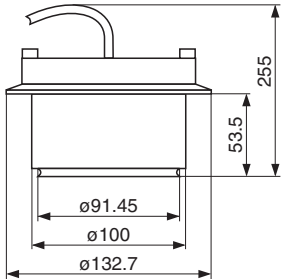
Sanitary tank spud with extension
