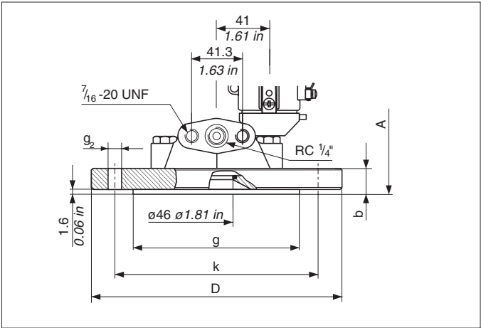
JIS flange 10 K 80 A, connection dimensions according to JIS B2210/B2238, contact face type: raised face RF
