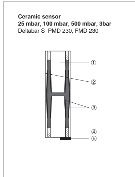
Ceramic sensor ① Basic body ② Diaphragm ③ Electrodes ④ Fritted glass ⑤ Temperature sensor
