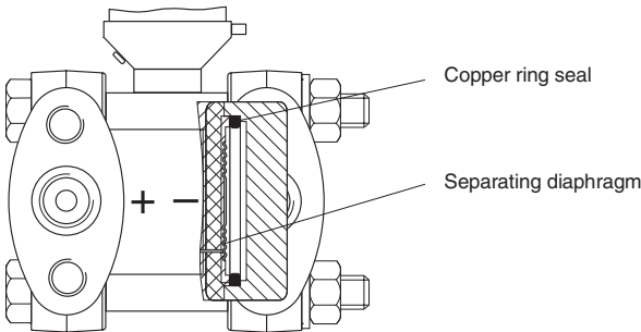
A Position of the copper ring seal
