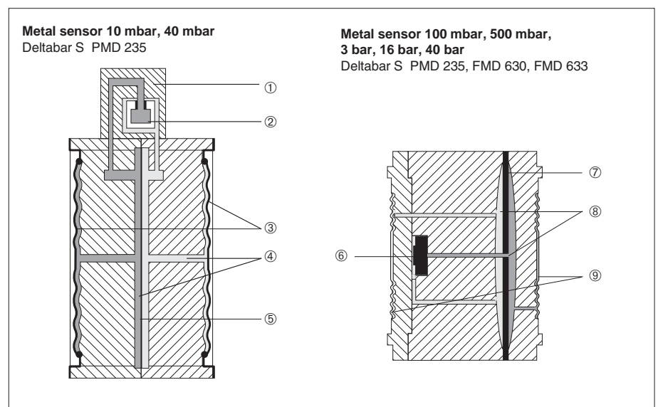
Metal sensor 10 mbar, 40 mbar ① Measuring element ② Silicon diaphragm ③ Separating diaphragm as nap diaphragm extended ④ fill fluid ⑤ Integrated overload protection Metal sensor 100 mbar, 500 mbar, 3 bar, 16 bar, 40 bar ⑥ Measuring element ⑦ Overload diaphragm ⑧ Fill fluid ⑨ Separating diaphragm as nap diaphragm extended
