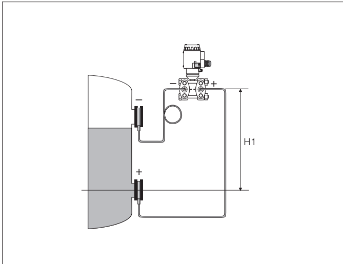
Installation above the lower diaphragm seal
