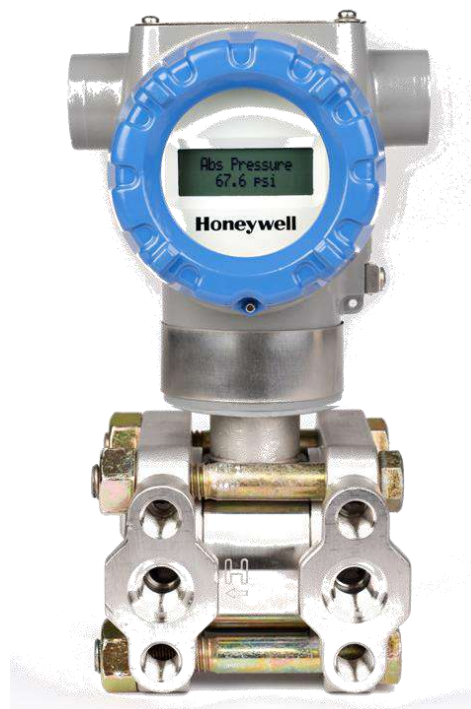
Figure 1 – STD700 Differential Pressure Transmitters feature field-proven piezoresistive sensor technology
