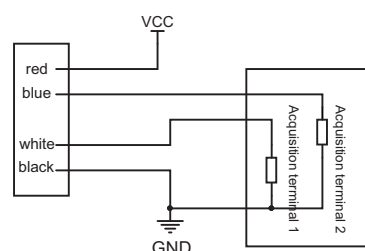
wiring diagram
