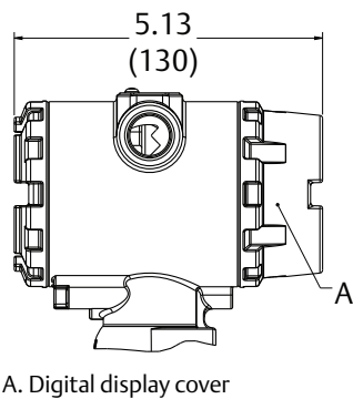
Figure 10. Rosemount 2051G with Optional Display
