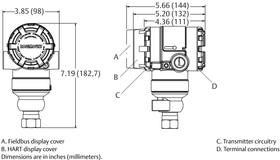
Figure 9. Rosemount 2051T
