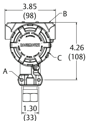
Figure 4. Rosemount 2088 Nameplate and Labels
