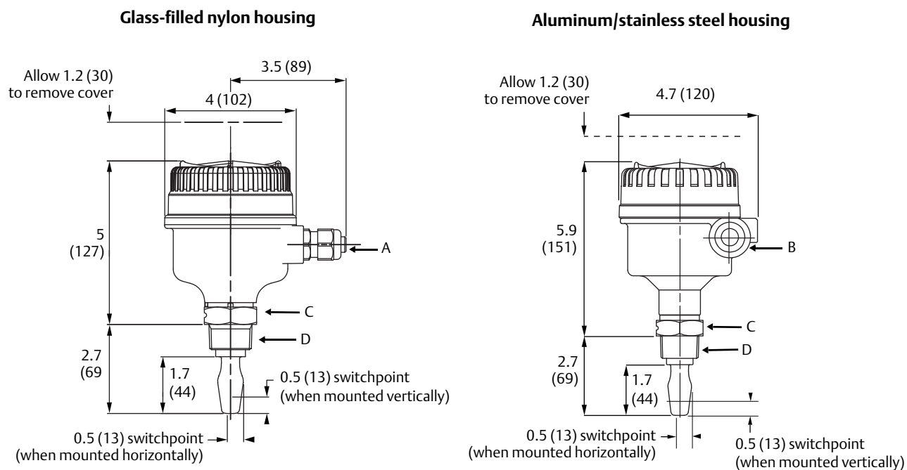
Figure 3. \frac{3}{4} - and 1-in. Threaded Mounting (Standard Length)
