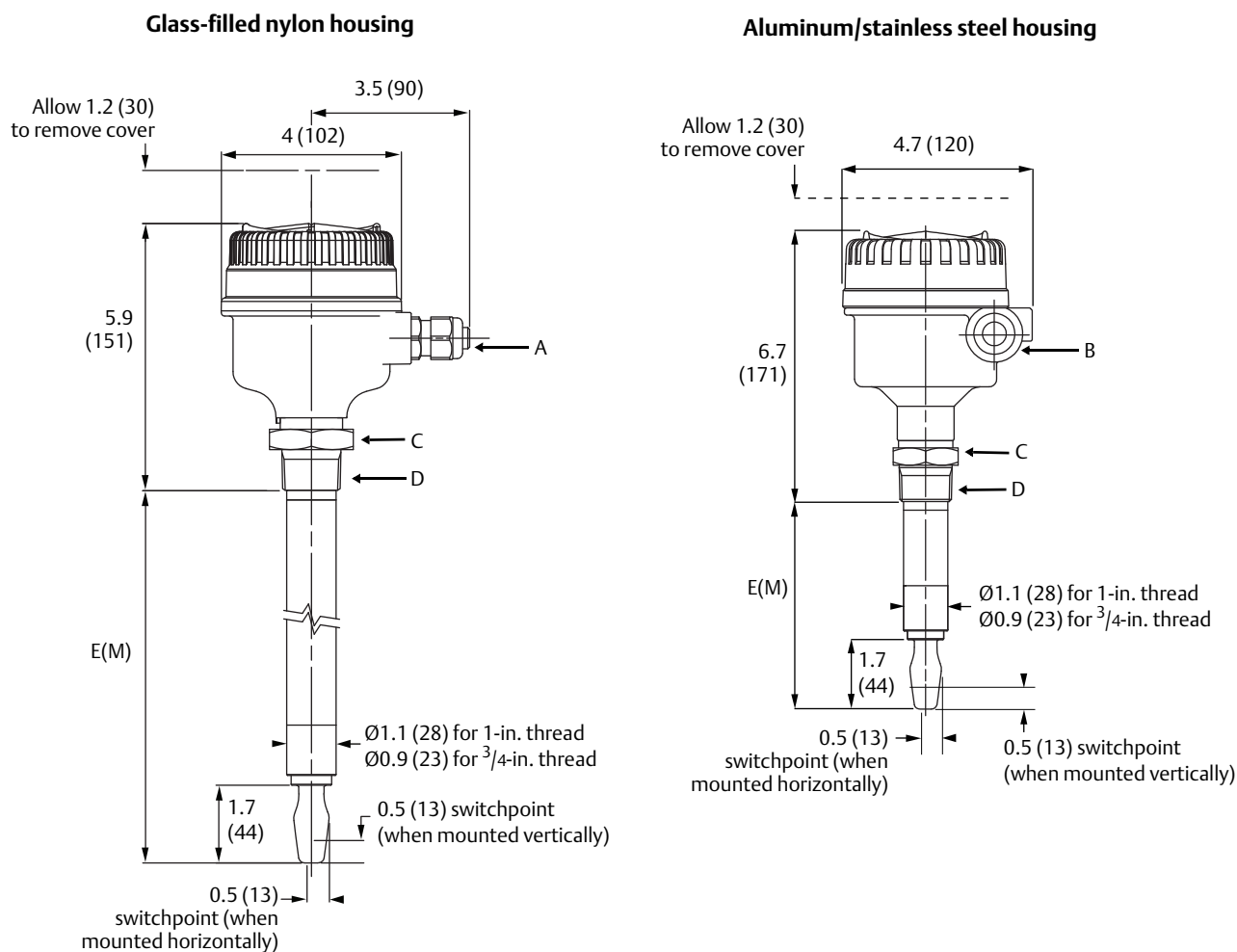
Figure 4. \frac{3}{4} - and 1-in. Thread Mounting (Extended Length)
