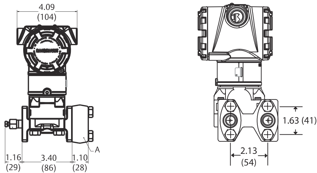
Figure 12: Rosemount 3051C Coplanar with Traditional Flange
