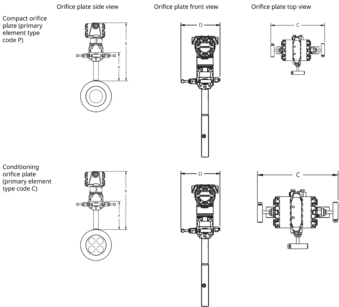
Figure 21: Rosemount 3051CFC Compact Orifice Flow meter
