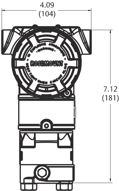
Figure 8: Rosemount 3051C Coplanar Flange
