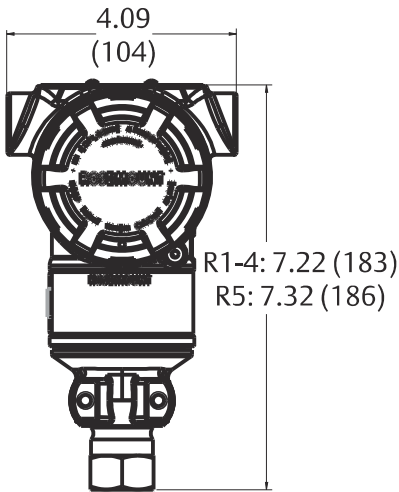
Figure 15: Rosemount 3051T
