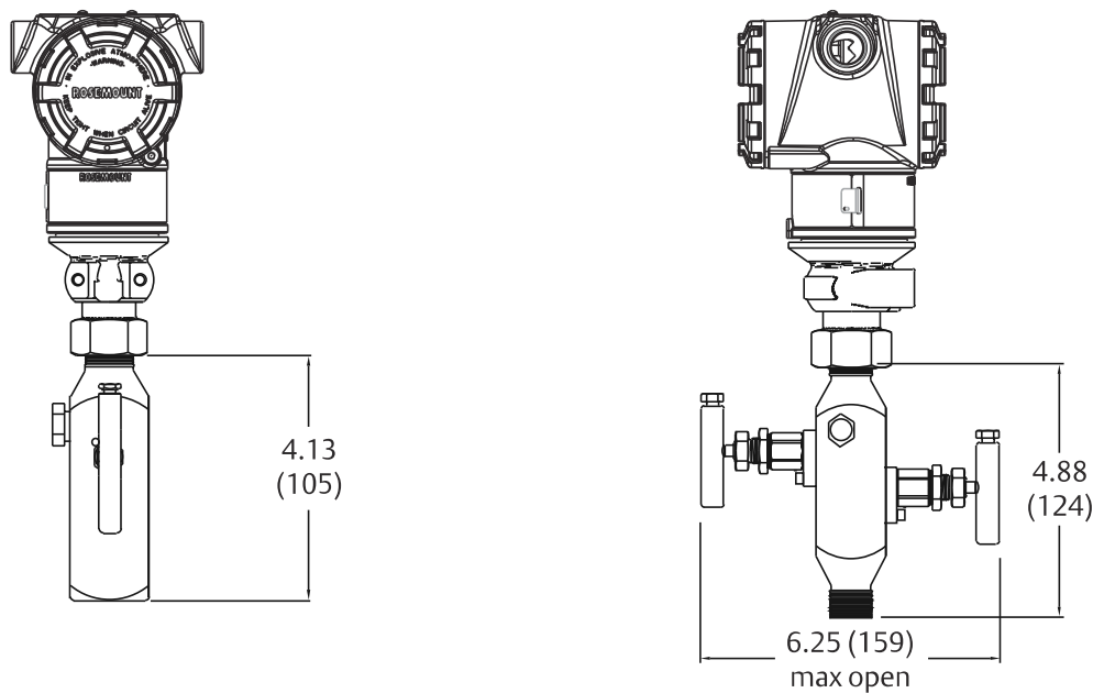
Figure 18: Rosemount 3051T with Rosemount 306 2-Valve Integral Manifold
