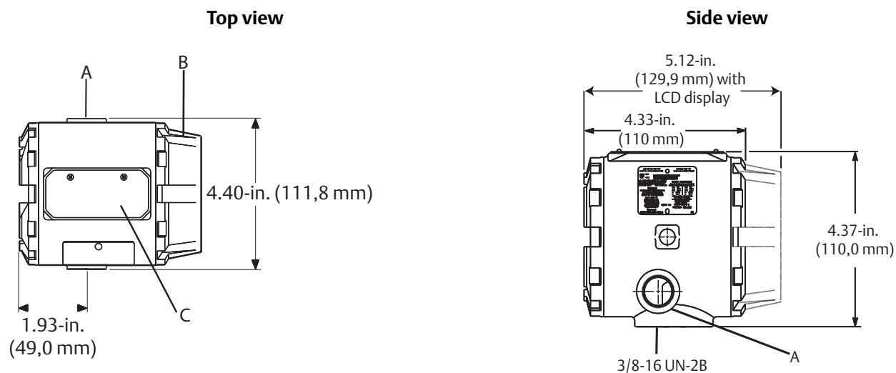
Figure 3. Transmitter
