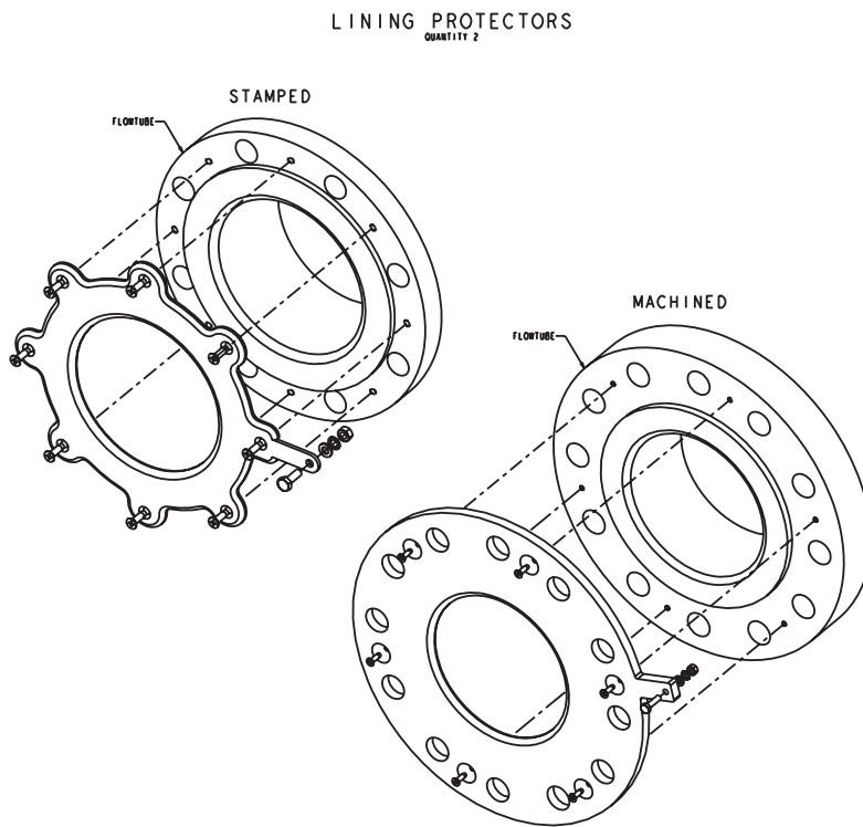
FIGURE 22. Liner Protectors
