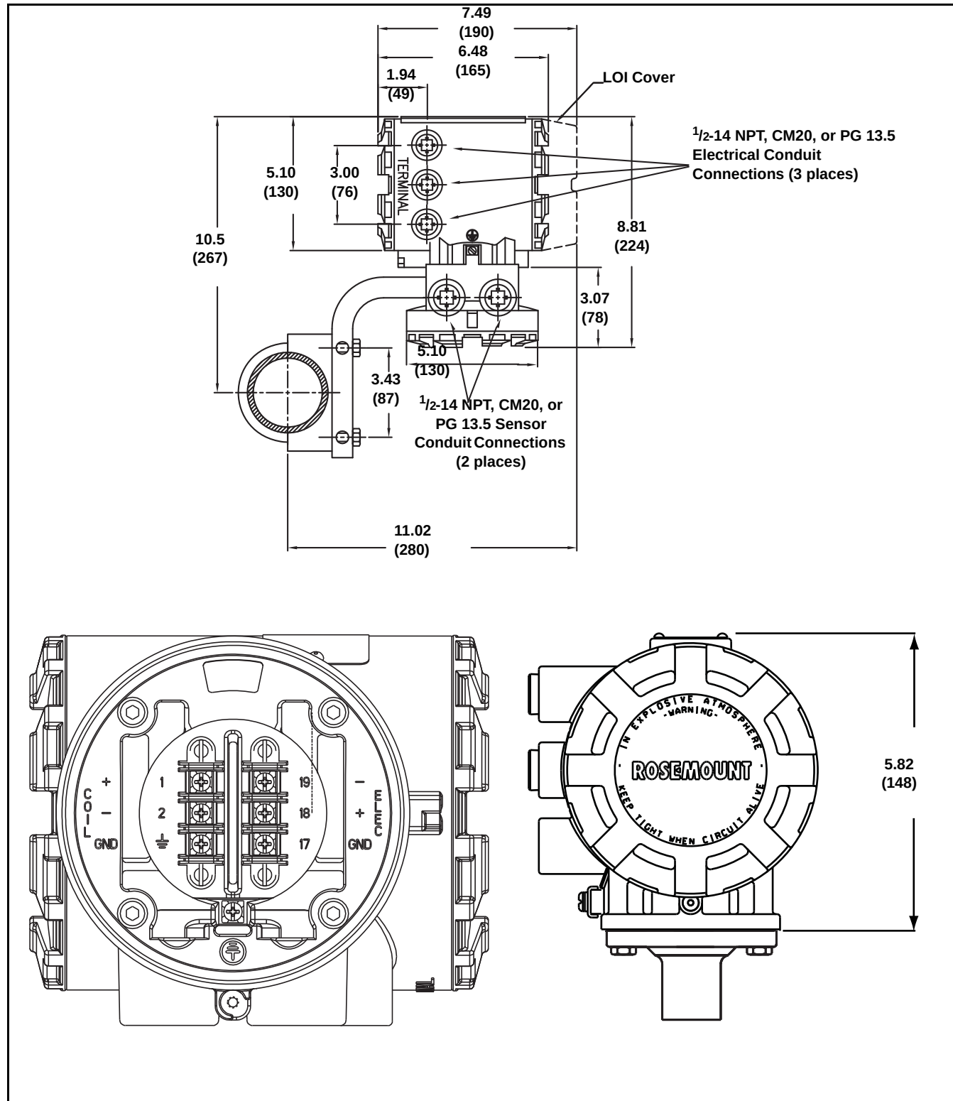
FIGURE 12. Rosemount 8732E Transmitter
