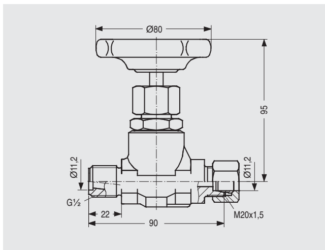
Shut-off valve 7MF9017-1B. and -2B.., dimensions in mm
