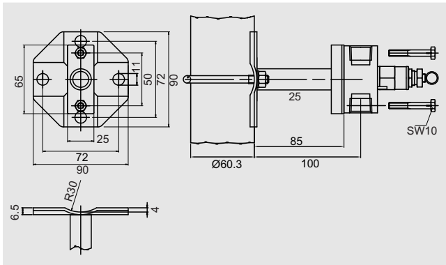
Mounting bracket (7MF9011-8AB) for shut-off valves 7MF9011-4DA and 7MF9011-4EA for wall, rack or pipe mounting, dimensions in mm
