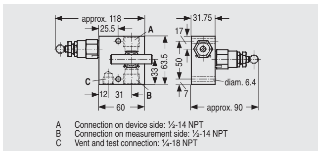
Double shut-off valve DN 5 (sleeve-sleeve) 7MF9011-4DA, dimensions in mm
