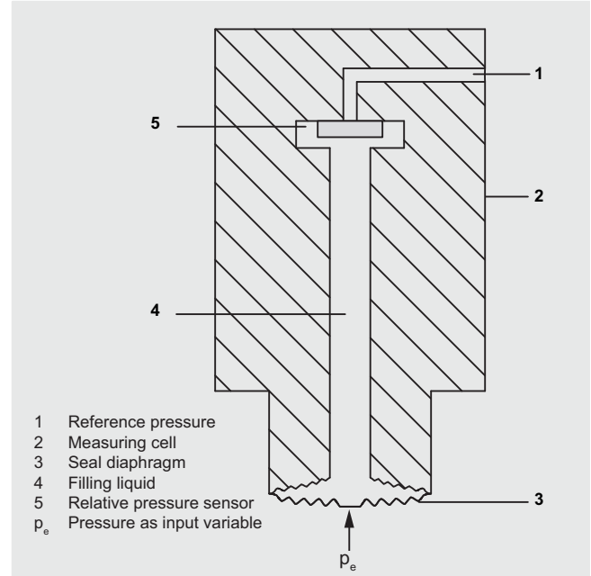
Measuring cell for gage pressure, front-flush diaphragm, function chart
