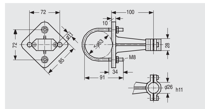
Instrument bracket form A, wall or pipe mounting, M56340-A0053/-A0079, dimensions in mm
