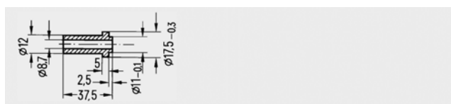
Nipple G \frac{1}{2} 7MF9007-4KA/-4LA, dimensions in mm
