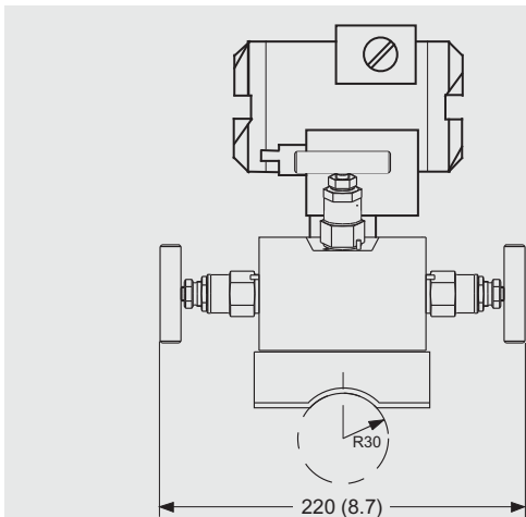
Valve manifold 7MF9411-5BA with mounted differential pressure transmitter, dimensions in mm (inch)
