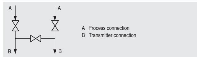
3-spindle valve manifold for vertical differential pressure lines, connections
