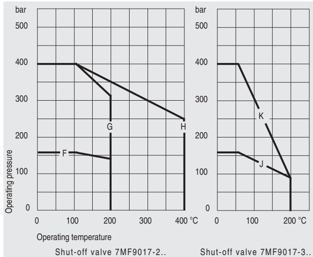
Shut-off valve 7MF9017-2.. and -3.., permissible working pressure as a function of the permissible working temperature
