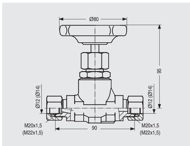
Shut-off valves 7MF9017-1C., -1D. and -2C.., dimensions in mm
