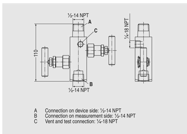
Double shut-off valve DN 5 (sleeve-collar) 7MF9011-4FA, dimensions in mm
