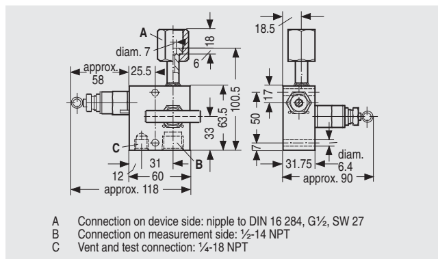
Double shut-off valve DN 5 (sleeve-nipple) 7MF9011-4EA, dimensions in mm
