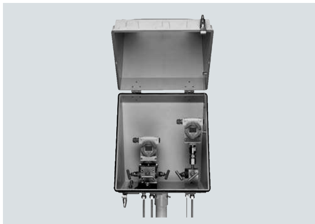
SITRANS P pressure transmitter for differential pressure, mounted in protective box (available on request)
