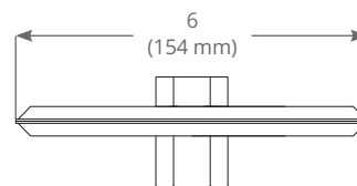
1/2 NPT Models 530-535
