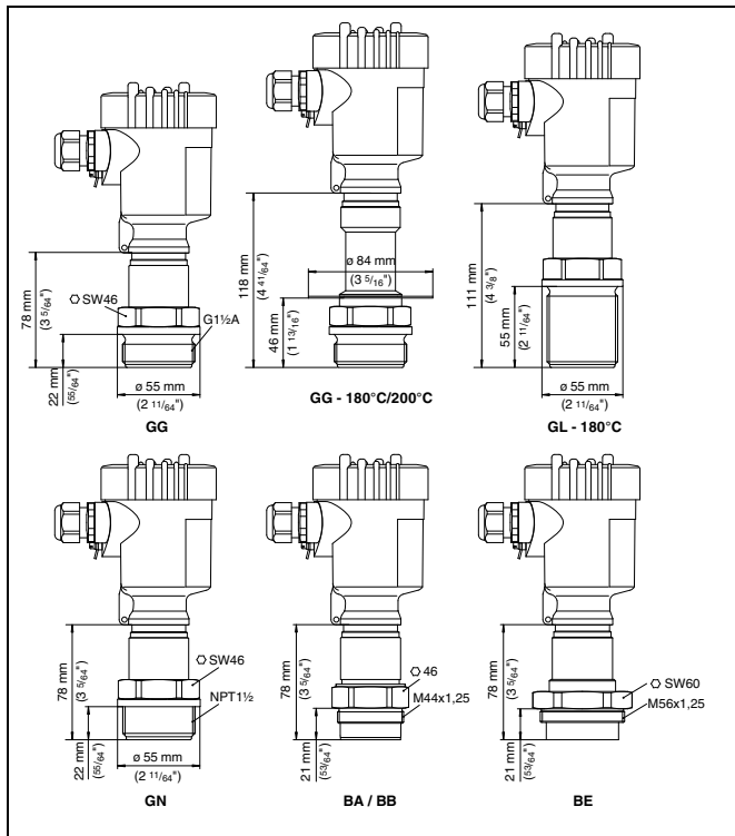
Fig. 39: VEGABAR 65 - threaded fitting: GG = G 1/2 A, GL = G 1/2 A thread length 55 mm, GN = 1 1/2 NPT, BA/BB = M44 x 1.25; BE = M56 x 1.25
