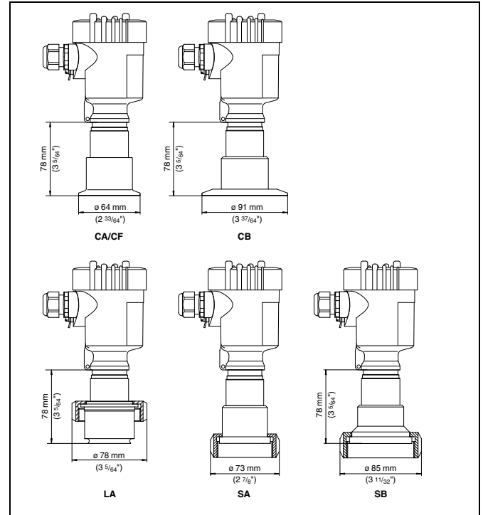
Fig. 40: VEGABAR 65 - hygienic fitting: CA/CF = Tri-Clamp 2 inch/Tri-Clamp 2 1/2 inch, CB = Tri-Clamp 3 inch, LA = hygienic fitting with compression nut F40, SA = SMS DN 38, SB = SMS DN 51
