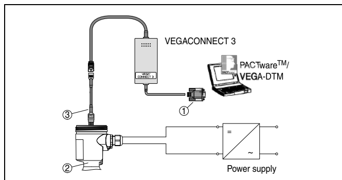
Fig. 17: Connection of the PC directly to the sensor via I²C interface
