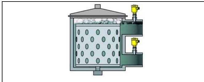
Fig. 9: Pressure measurement on a screen with VEGABAR 64
