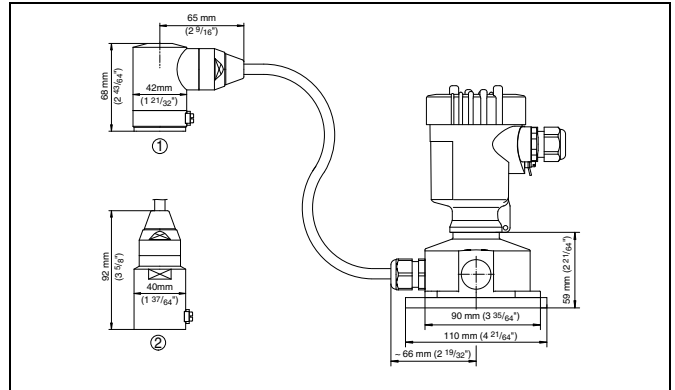
Fig. 25: Transmitter and remote housing with IP 68 version
