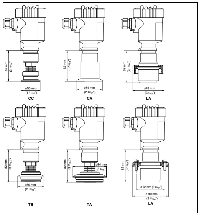
Fig. 30: VEGABAR 63 CC = Tri-Clamp 1 1/2", CA = Tri-Clamp 2", LA = hygienic fitting with compression nut, TB = Tuchenhausen Varivent DN 25, TC = Tuchenhausen Varivent DN 32, AA = DRD
