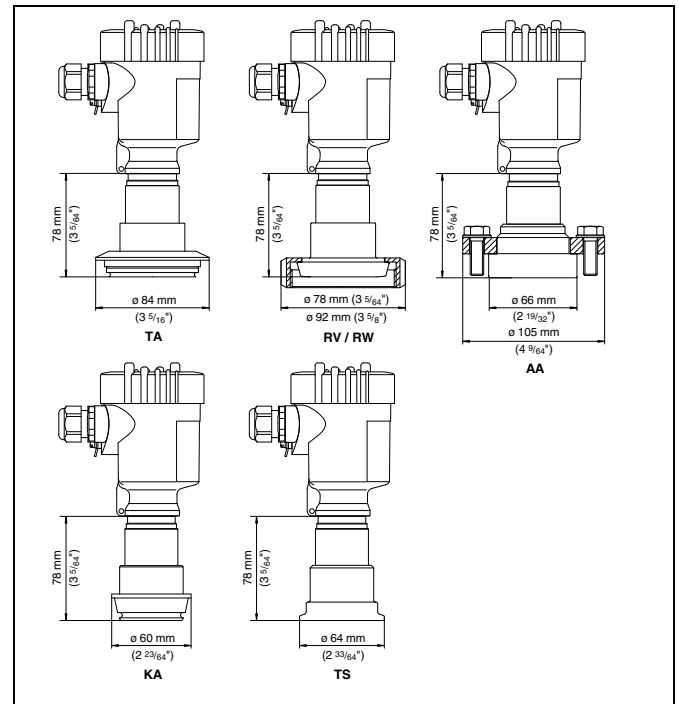
Fig. 41: VEGABAR 65 - hygienic fitting: TA = Tuchenhagen Varivent DN 32, RV/RW = bolting DN 40/DN 50 according to DIN 11851, AA = DRD, KA = conus DN 40
