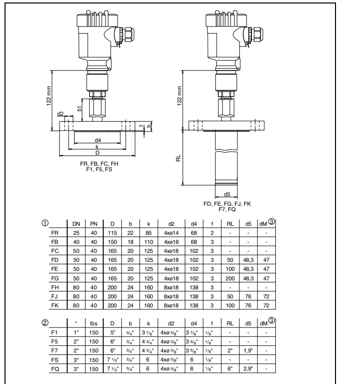
Fig. 26: VEGABAR 61 - flange version
