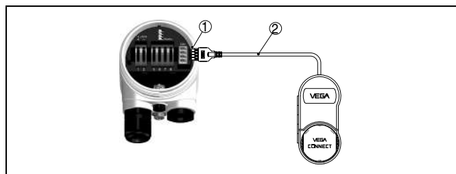
Fig. 19: External connection of the PC directly to the sensor via I²C interface
