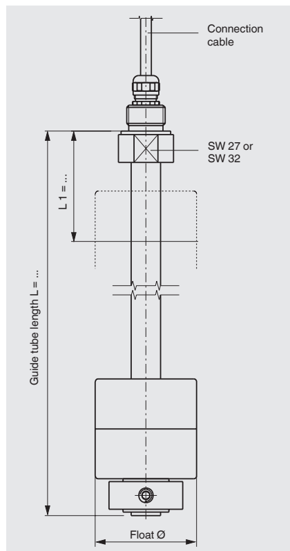
Mounting thread and connection cable
