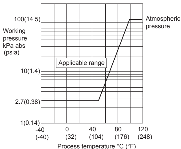
Figure 1-2. Working Pressure and Process Temperature [For EJX630A]
