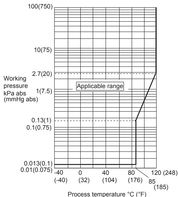
Figure 1-1. Working Pressure and Process Temperature [For EJX610A]
