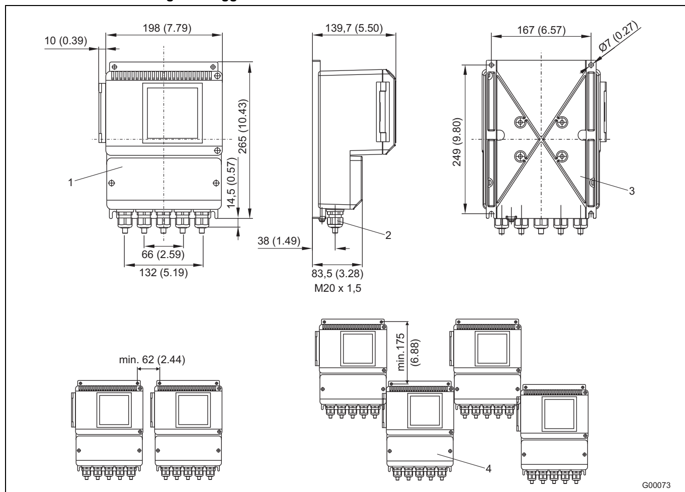
Fig. 30: Dimensions in mm (inch)
